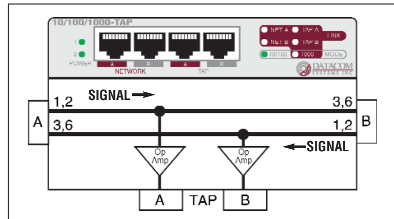
10/100 BaseT Functional Diagram
